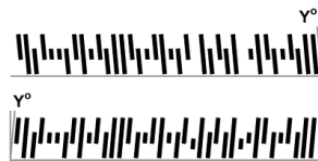
Figure 17 – 4-State Mailmark Barcode Bar Skew Y (Not to Scale)
