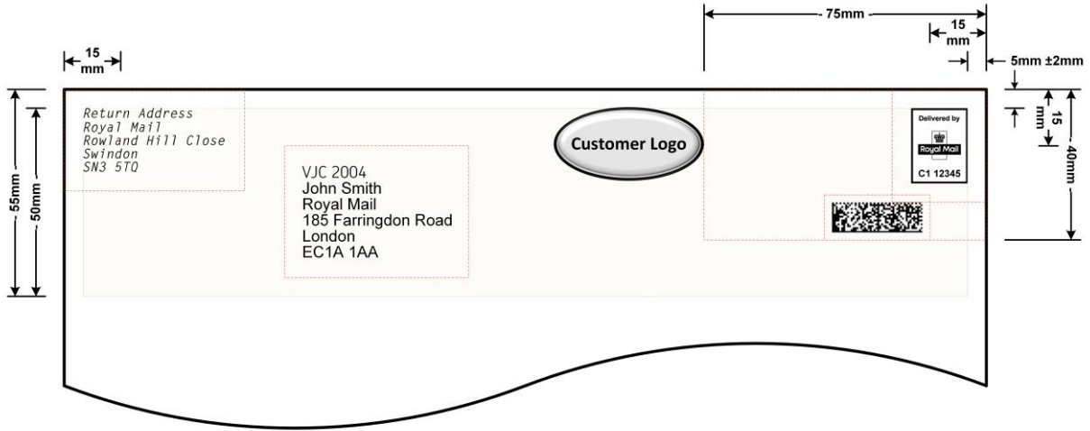
Figure 52 – Large Letter Paper Wrap – Printing (Not to scale)
